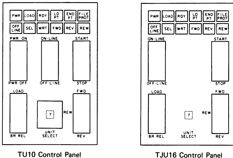
Figure 23-9 Control Panels
