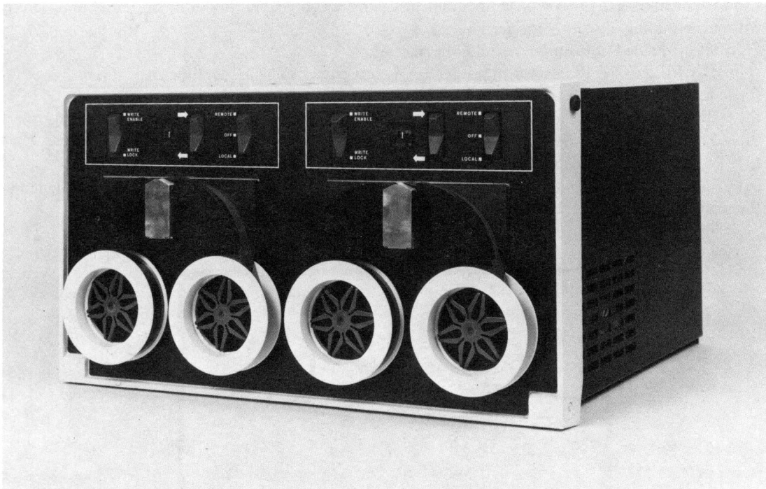
Figure 23-7 TU56 DECTape Transport
