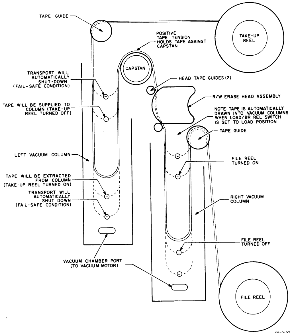
Figure 23-10 Magtape Transport Threading Diagram
