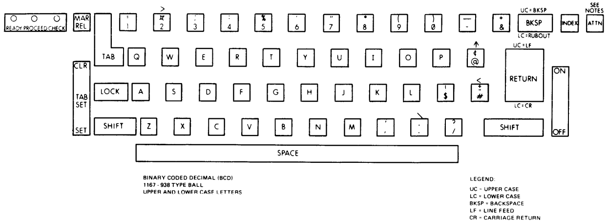
Figure 23-15 BCD Keyboard
